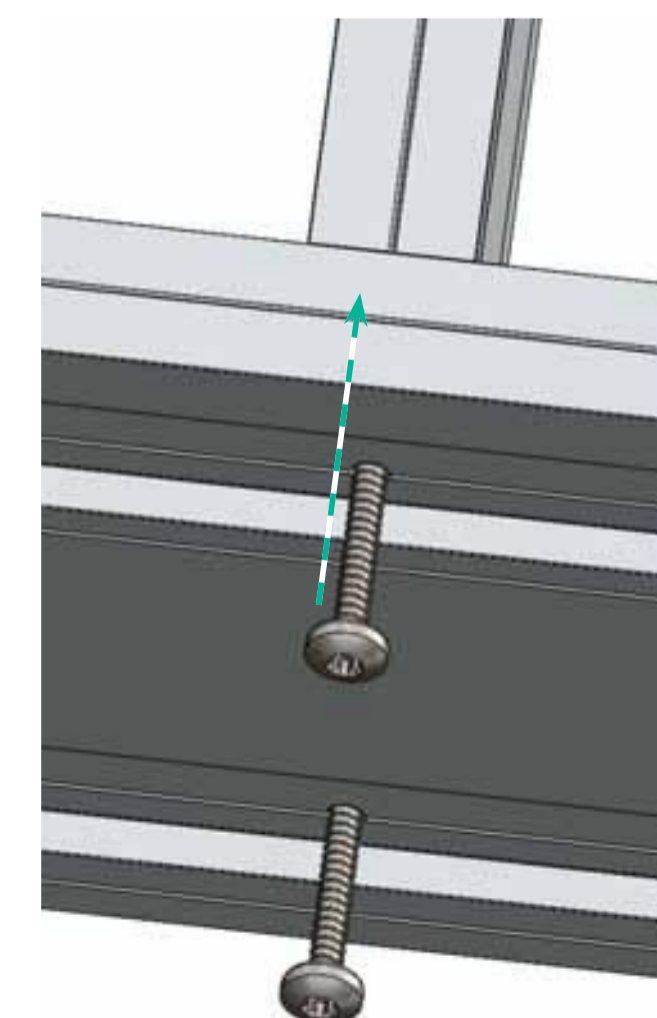
Fix joist to beam
