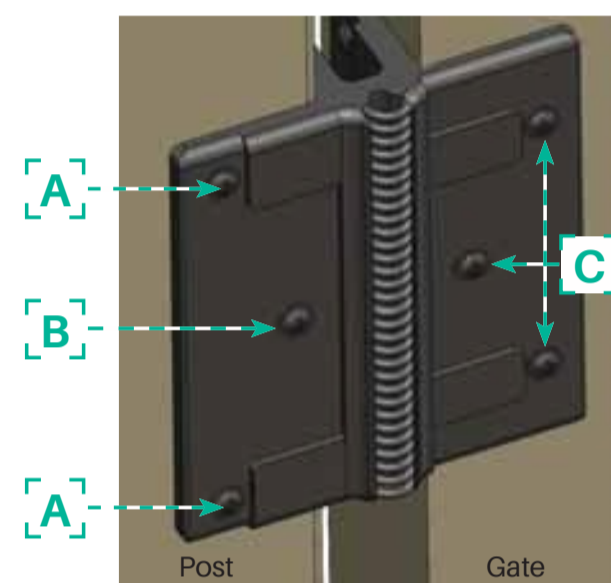
Fix DALHINGE to gate / post
