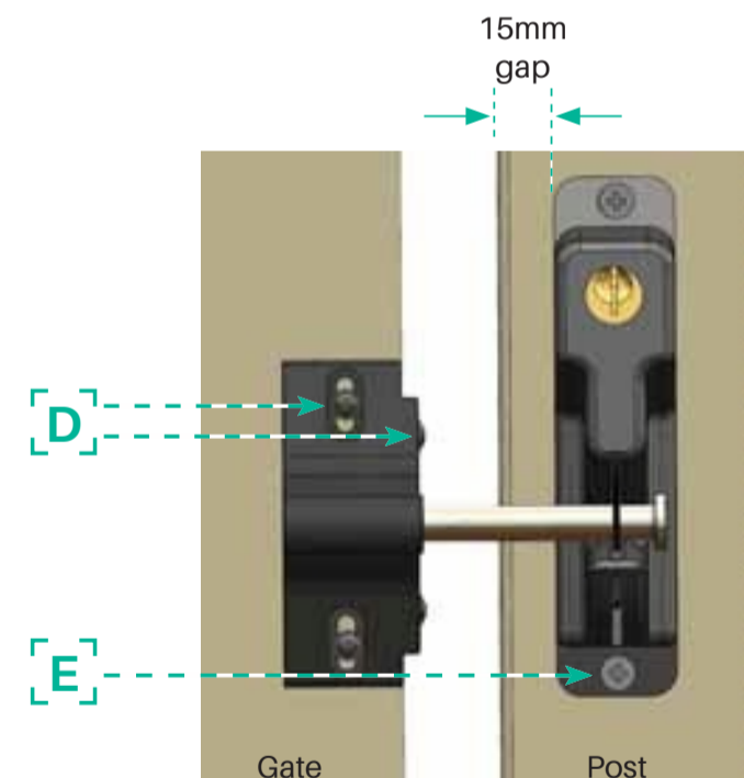
Fix DALLATCH assembly to gate / post
