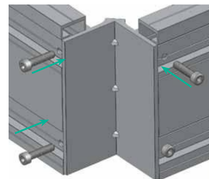
Fix using socket head cap screws
