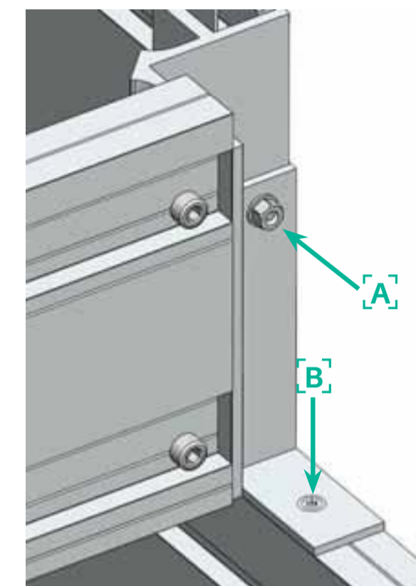
Position the L Bracket and fix through the corner bracket
