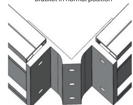
Bracket in normal position
