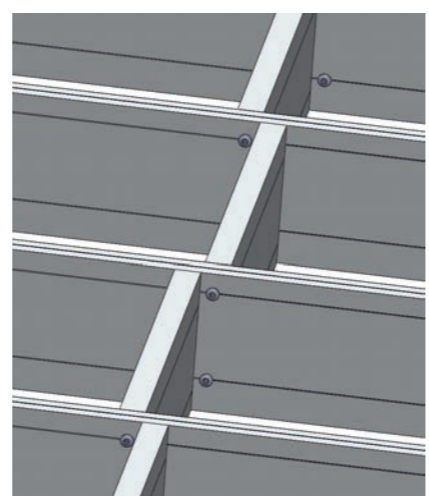
Noggins should be staggered to allow for fixings
